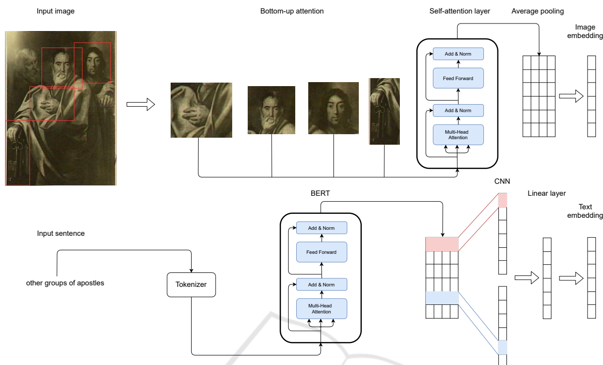
Figure 1: The scheme of the SAEM framework. The upper branch processes visual information and the lower branch is responsible for textual information.
