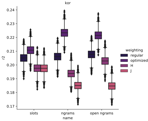
Figure 4: The R^2_{adj} , bootstrapped over 10,000 samples.
