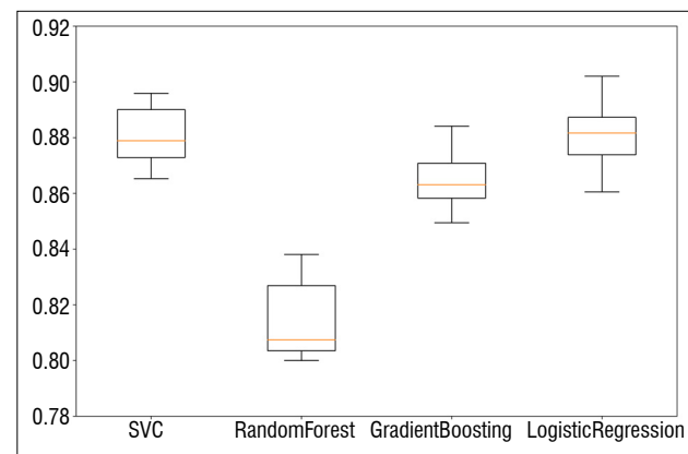
Figure 2: Accuracy scores.
