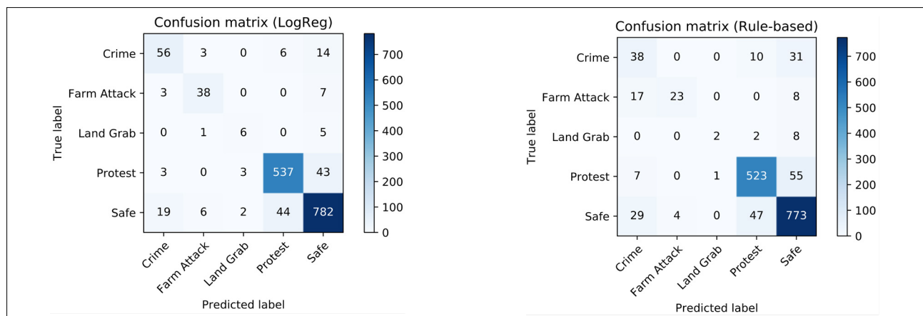
Figure 3: Confusion matrixes.
