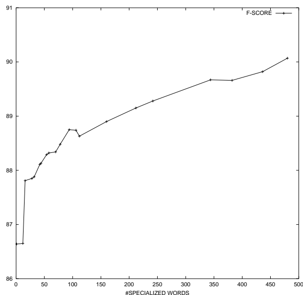
Figure 2: F-score as a function of the number of specialized words in the ILM
