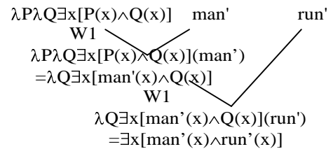
figure 3 : semantic translation of tree n°1
