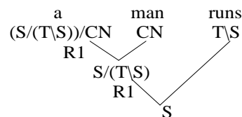
figure 1 : analysis tree n° 1
