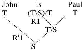
figure 2 : analysis tree n°2
