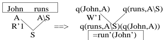
figure 6 : hypothesis H1
